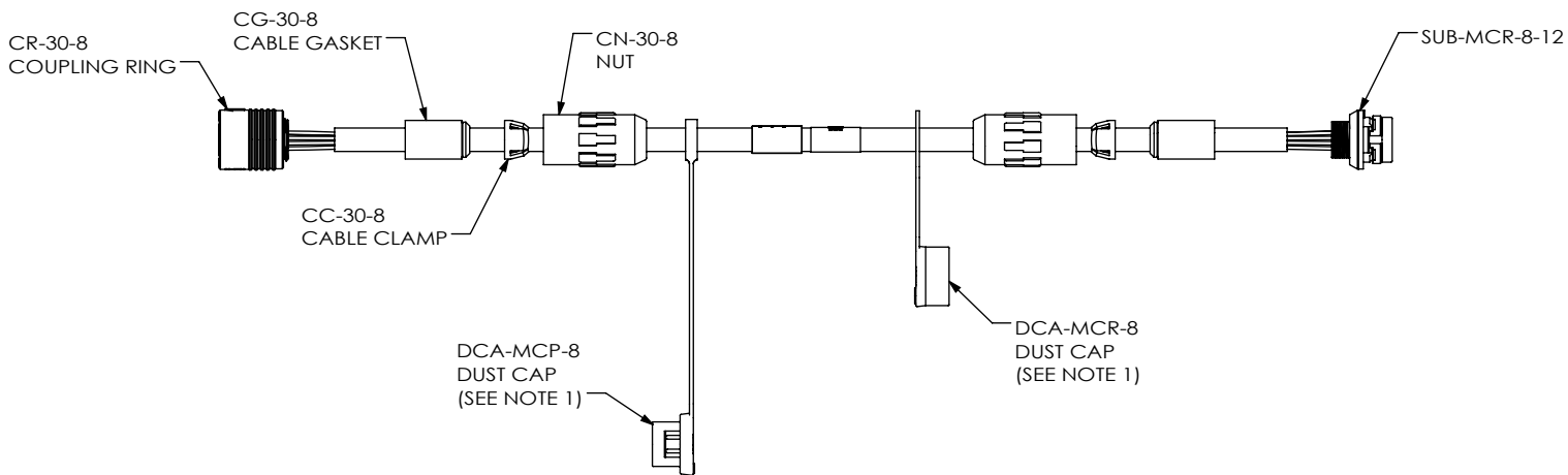
MCP-8-02-X-XX.XX-T-S WITH DUST CAP SHOWN
